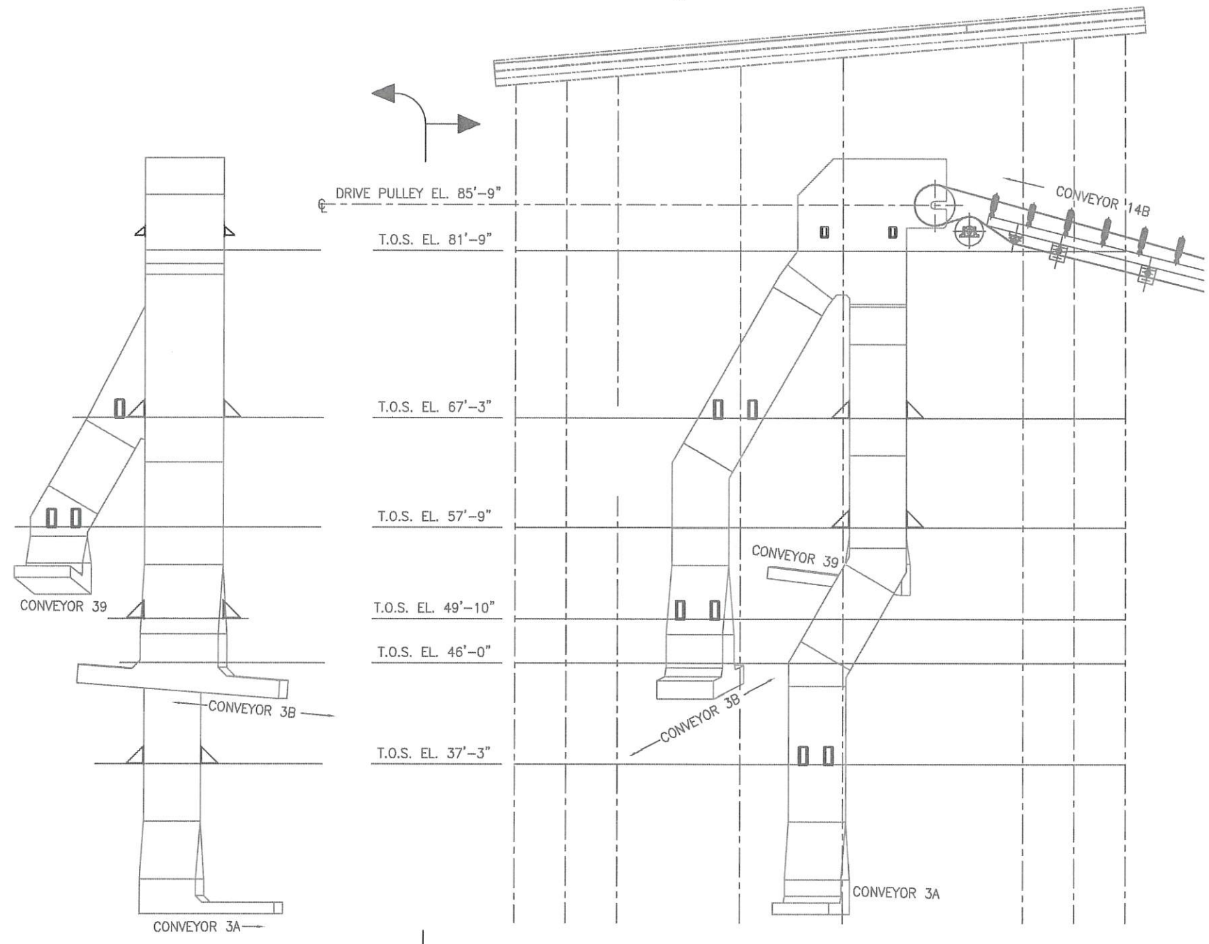
T-24 VIEW A-A
